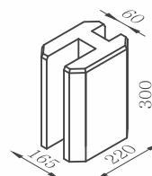
ŁDP30 straight connector
