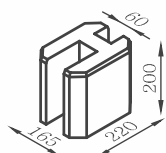
ŁDP20 straight connector
