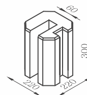
ŁDN30 corner connector
