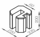
ŁDN20 corner connector
